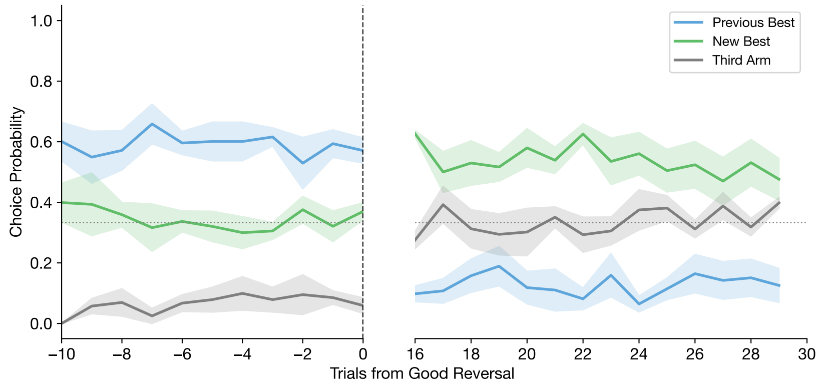
Good Reversal-Aligned Choices (mean \pm se across subjects | n=5 subjects, n=52 reversals) (Skipping first 15 trials post-reversal)
